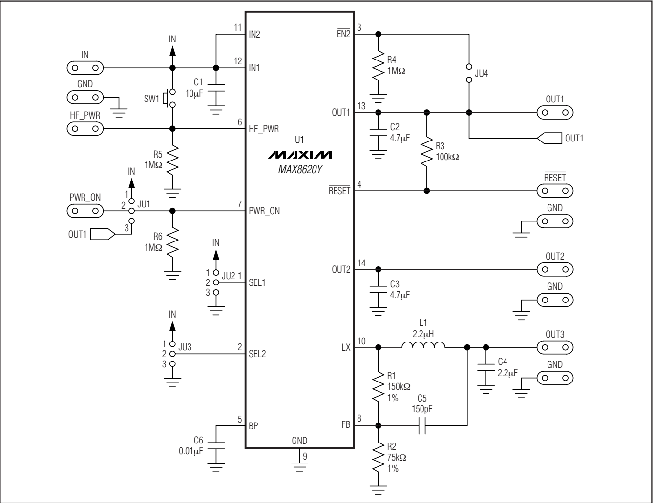
Figure 1. MAX8620Y EV Kit Schematic
